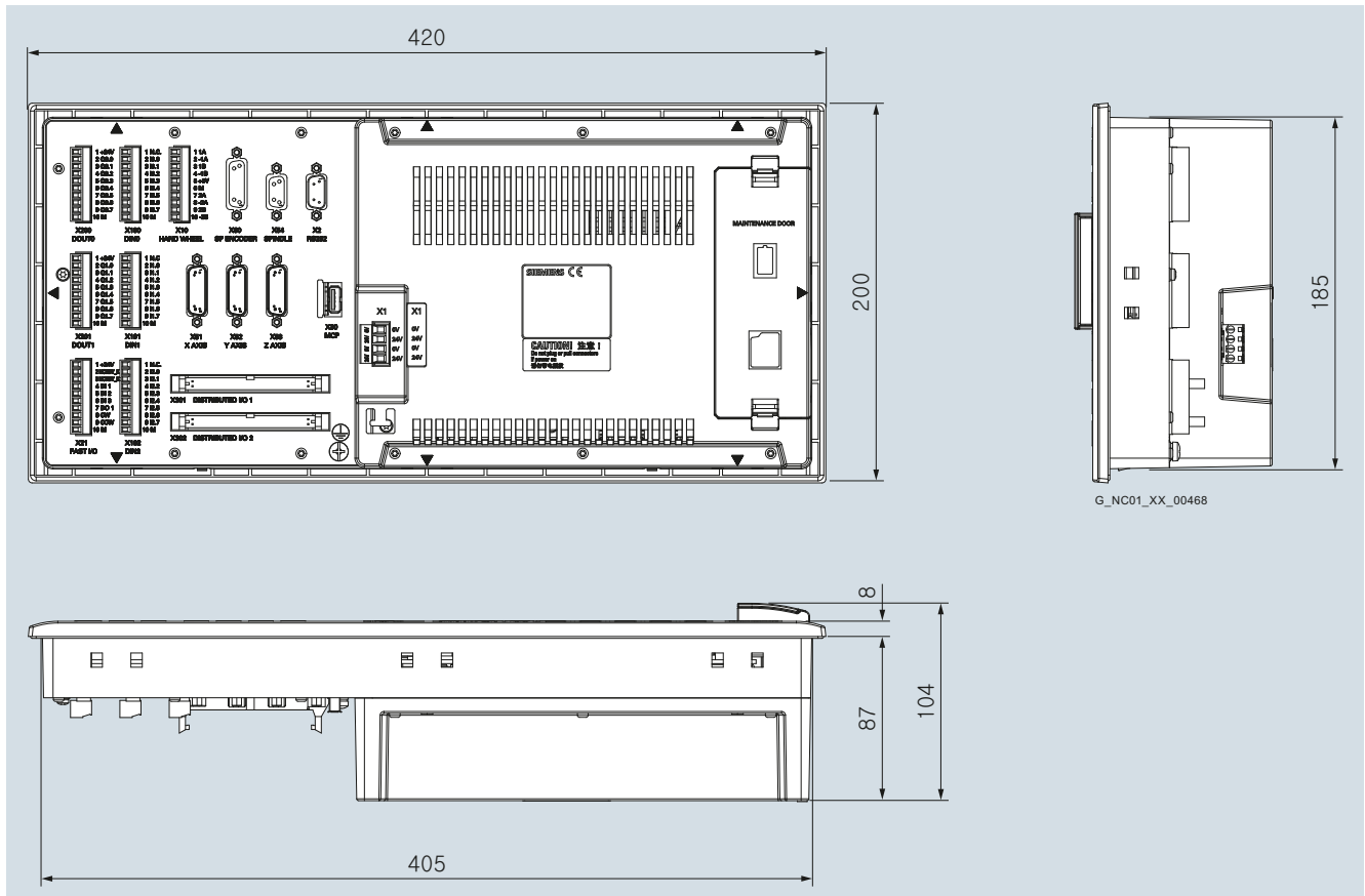
SINUMERIK 808D Turning/Milling PPU 141.1 horizontal
