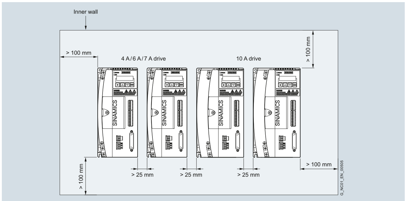
Mounting clearance
