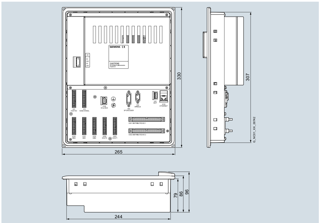
SINUMERIK 808D ADVANCED T/M PPU 160.3 vertical
