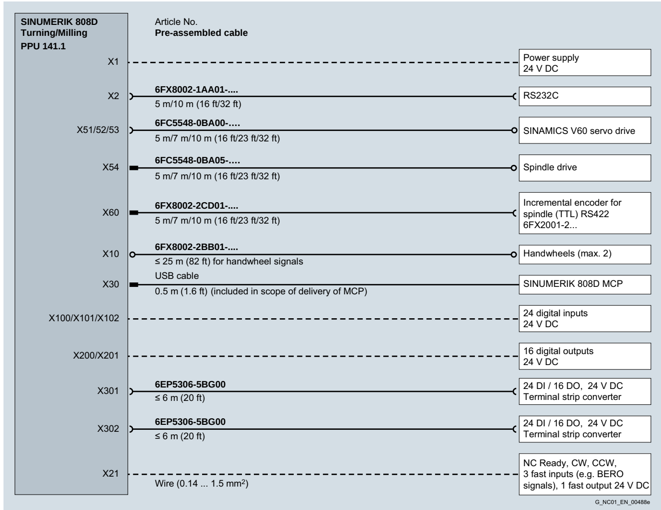
Connection overview of SINUMERIK 808D Turning/SINUMERIK 808D Milling PPU 141.1
