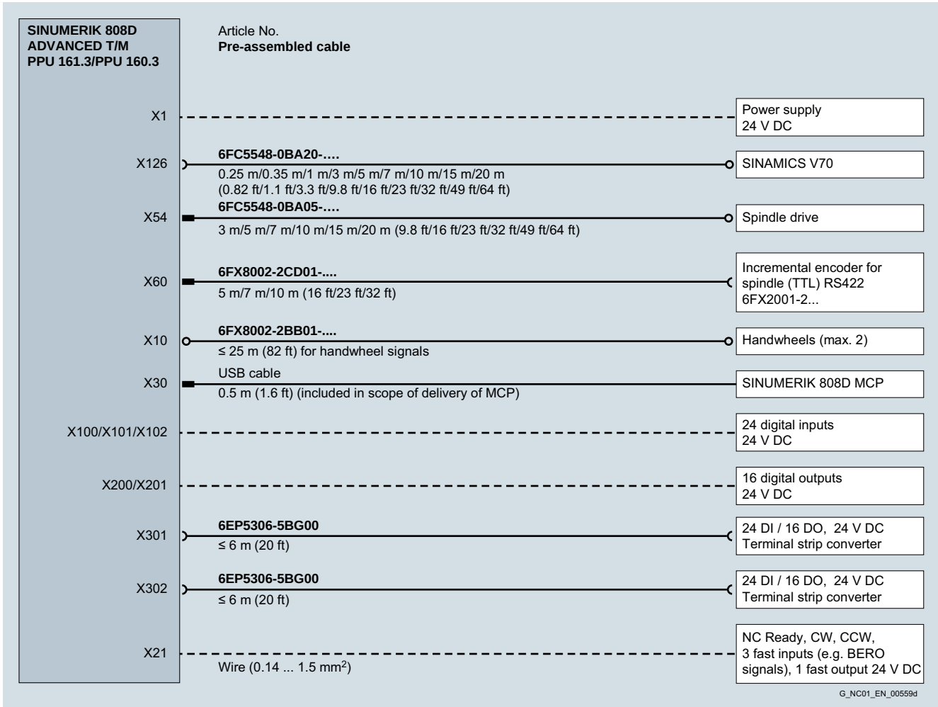
Connection overview of SINUMERIK 808D ADVANCED T/SINUMERIK 808D ADVANCED M PPU 161.3/PPU160.3
