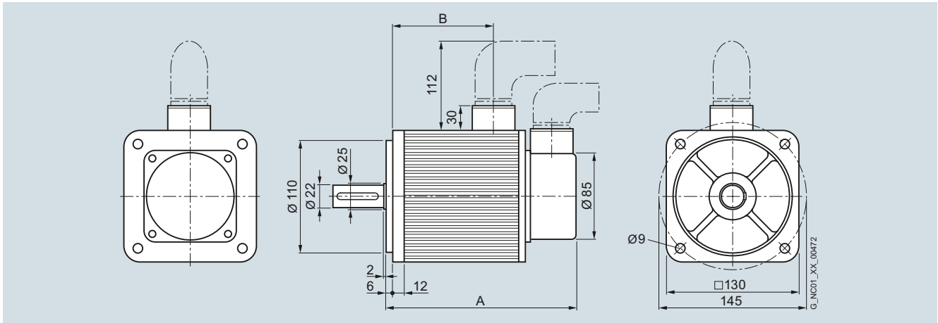
SIMOTICS S-1FL5 feed motor
